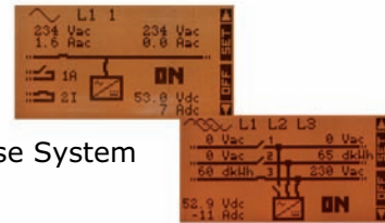
3 Phase System
