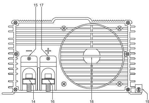
Fig. 6.1 (c) SWI 3000, Trasera.
