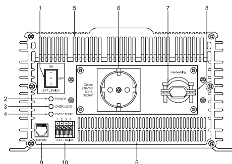
Fig. 6.1 (a) SWI 3000, Delantera.
